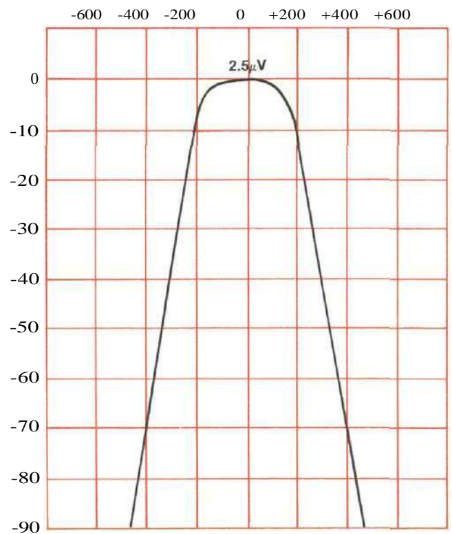
MR 500 SELECTIVITY
